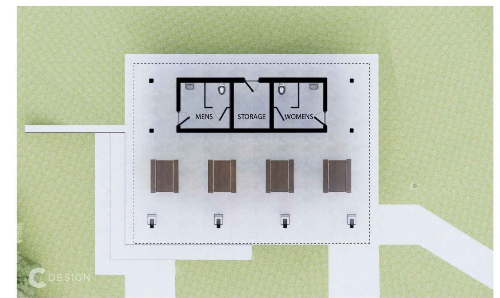
Shelter - Plan View
